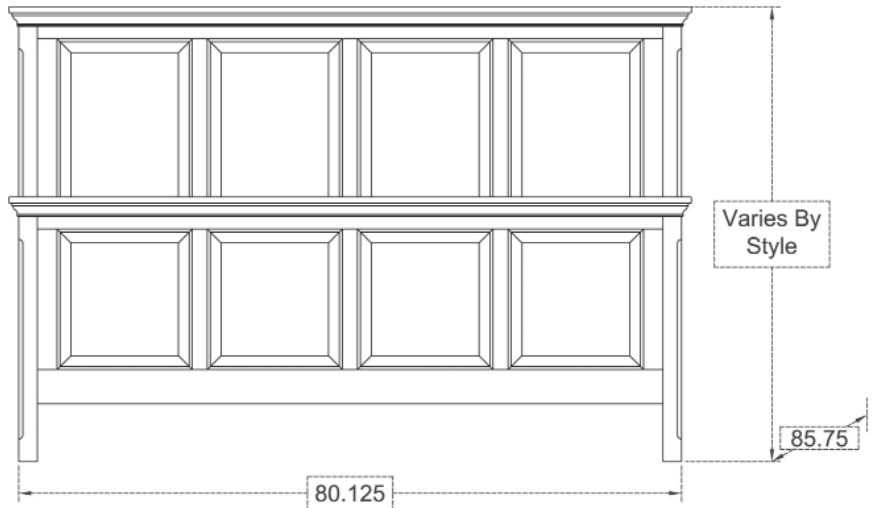
Exterior View by Style Standard size with molding on: 1 side | 2 sides
